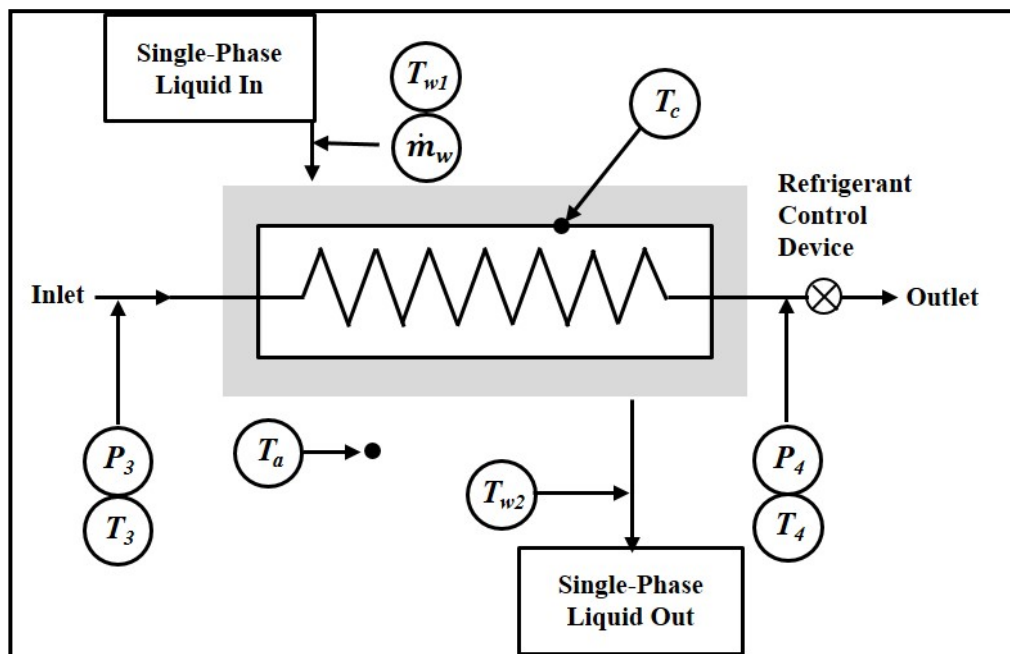
FIGURE 8: Condenser Calorimeter Method
