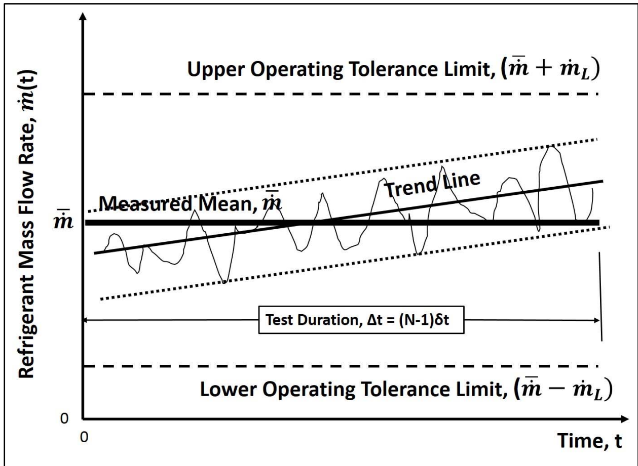
FIGURE 1: Graphical illustration of the method for determining the steady-state refrigerant mass flow rate criteria for test points
