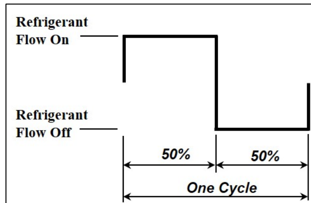
FIGURE 3: Theoretical cycle of refrigerant flow rate for a pulse-width modulated compressor that delivers 50% load
