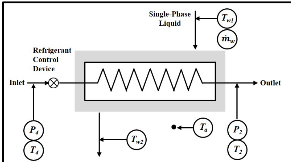
FIGURE 5: Secondary Fluid Calorimeter That Uses a Single-Phase Liquid
