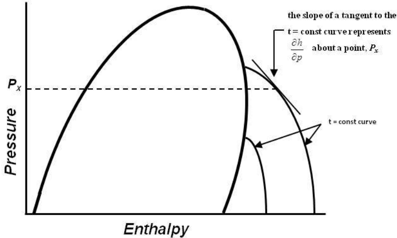
FIGURE A-1 Refrigerant Pressure-Enthalpy Diagram
