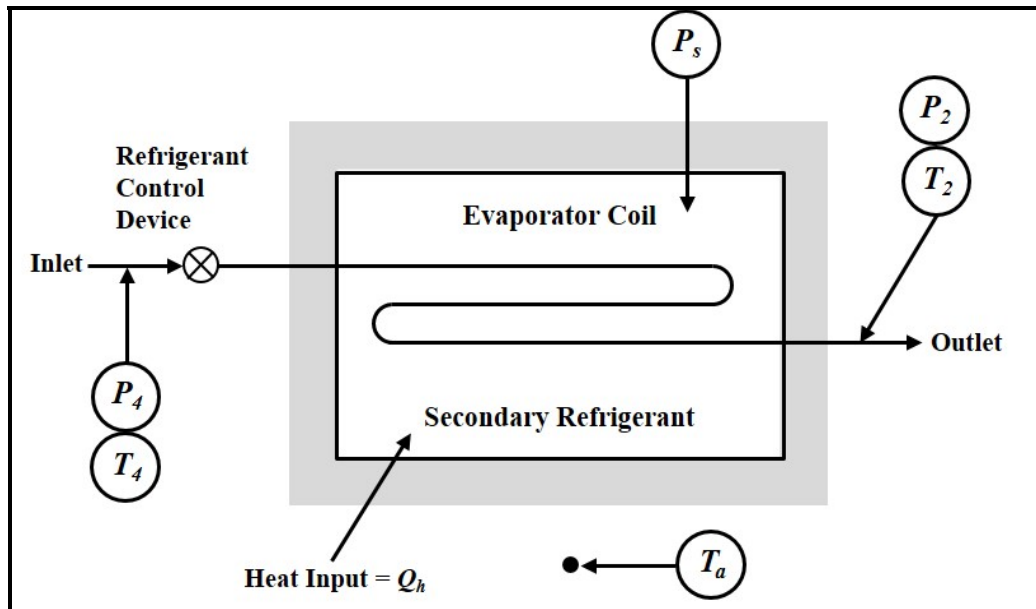
FIGURE 4: Secondary Refrigerant Calorimeter Method
