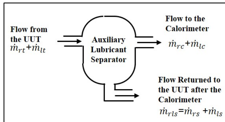
FIGURE 9: Auxiliary Lubricant Separator Schematic
