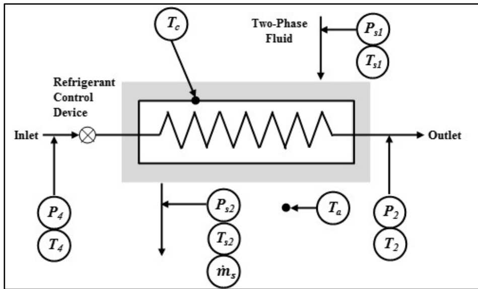
FIGURE 6: Secondary Fluid Calorimeter That Uses a Two-Phase Fluid
