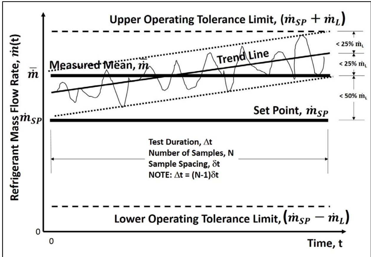
FIGURE 2: Graphical illustration of the method for determining the steady-state refrigerant mass flow rate criteria for targeted set points
