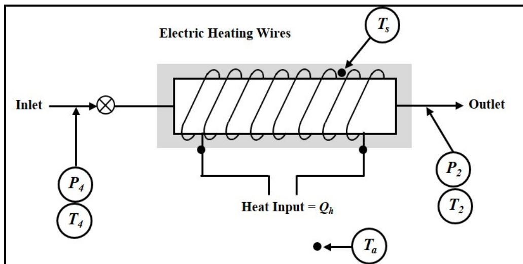
FIGURE 7: Primary Refrigerant Calorimeter Method
